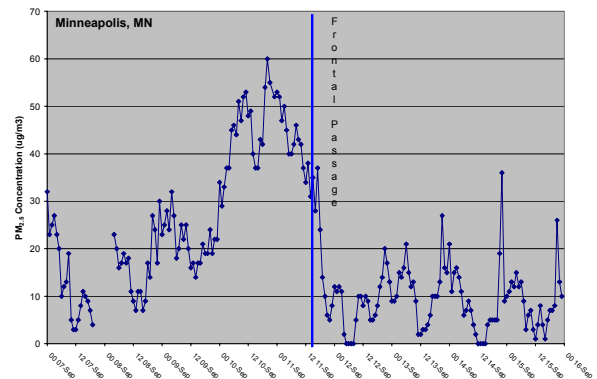
Figure 9. Average hourly PM 2.5 measurements for Minneapolis, Minnesota, from September 7 to 16. The timing of the frontal passage is marked by a blue line.
