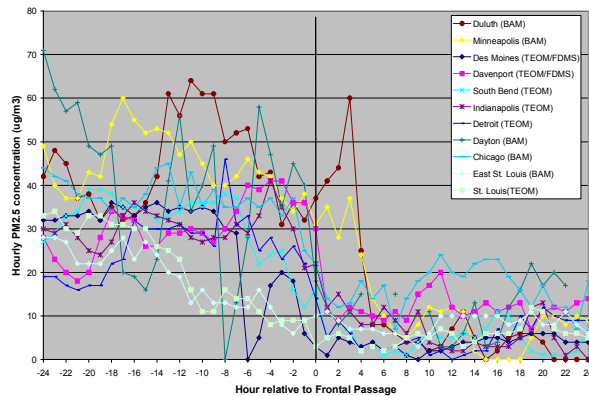
Figure 16. Front-relative PM 2.5 hourly concentrations for 11 Midwestern cities for 24 hours preceding and following the frontal passage. The types of instruments are identified; BAMs and TEOMs are present in the graph.
