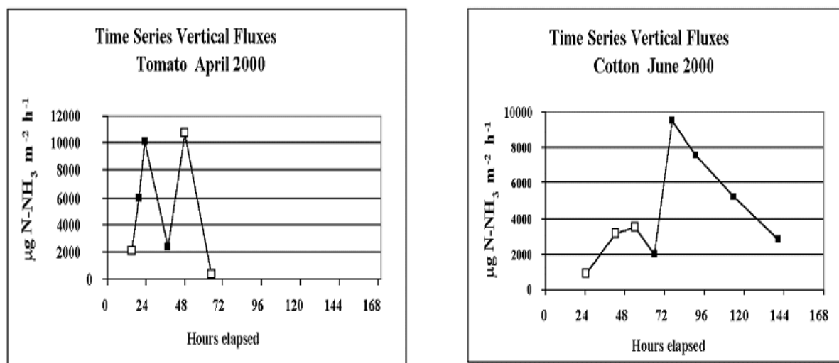
Figure 3-7. Ammonia emissions measured following fertilizer application from tomato (left) and cotton (right) fields ( http://geo.arc.nasa.gov/sge/casa/california.html ).
